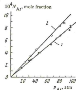
Figure 4. Solubility of argon as a function of gas pressure in 1) benzene and 2) toluene
